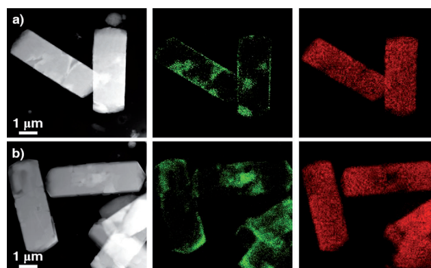
Figure 2. TEM images (left) and Ga (middle) and Al (right) TEM elemental mapping. The solid products obtained after heating the almost fully ordered Al-NAT zeolite (i.e., PST-4) in the Ga-NAT-ML solution at 150 °C for a) 3 and b) 14 days. The mappings show that no migration into the core occurs when the Al-NAT zeolite is already ordered.
